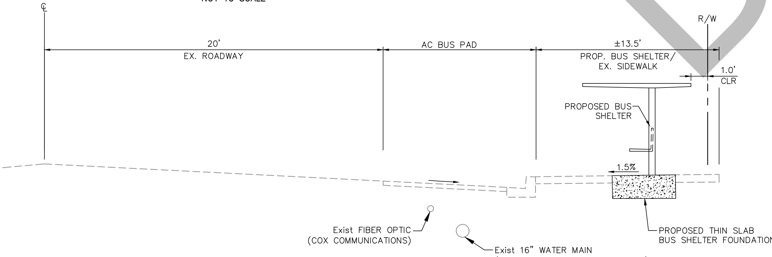
SECTION H-H NOT TO SCALE
