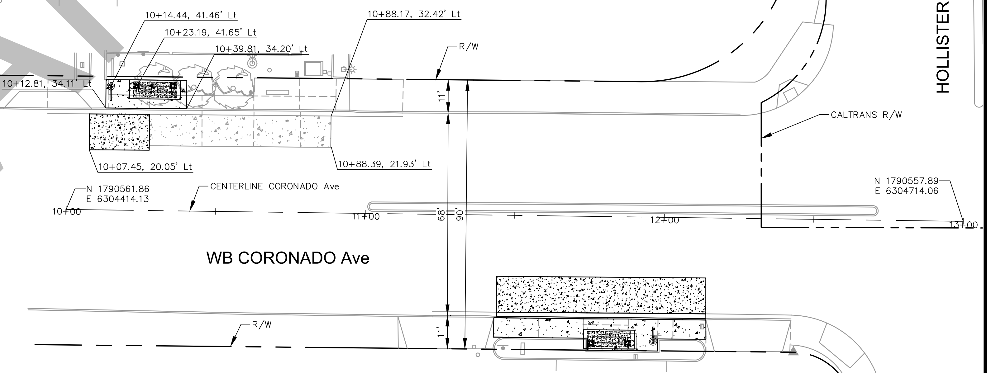
SURVEY CONTROL POINT LOCATION SCALE: 1" = 20'
